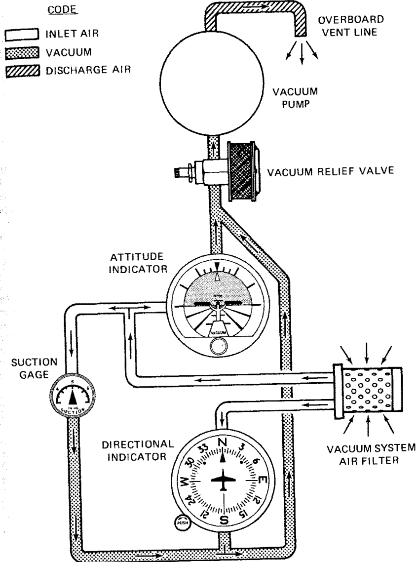
Figure 7-9. Vacuum System
