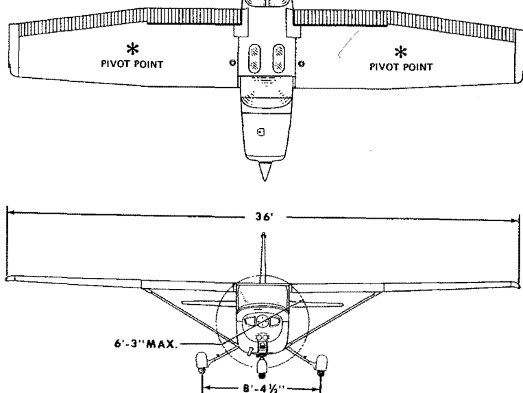
Figure 1-1. Three View
