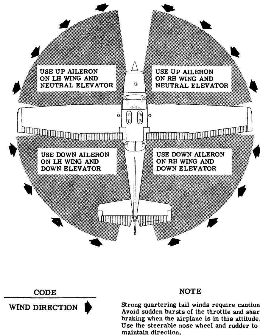
Figure 4-2. Taxiing Diagram
